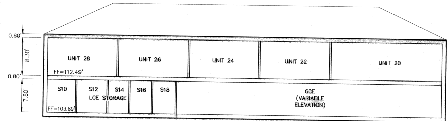
BUILDING 2613 SCALE: 1"=10'
