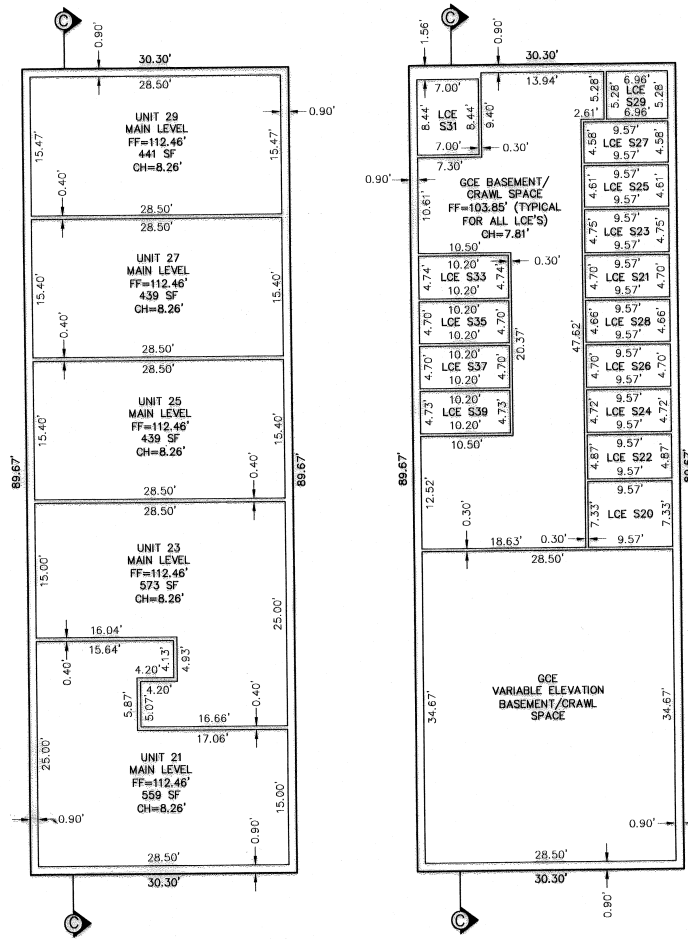
BUILDING 2621 SCALE: 1"=10'
