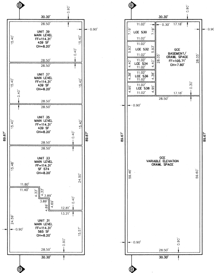
BUILDING 2633 SCALE: 1"=10'
