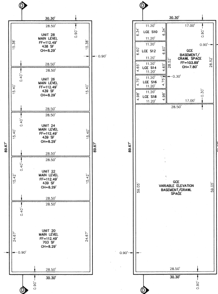
BUILDING 2613 SCALE: 1"=10'
