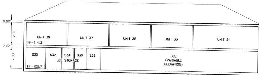
BUILDING 2633 SCALE: 1"=10'
