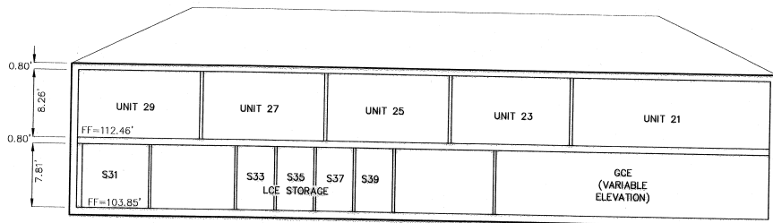
BUILDING 2621 SCALE: 1"=10'
