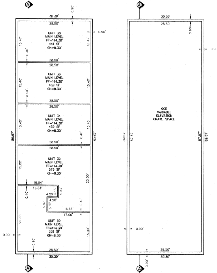
BUILDING 2643 SCALE: 1"=10'
