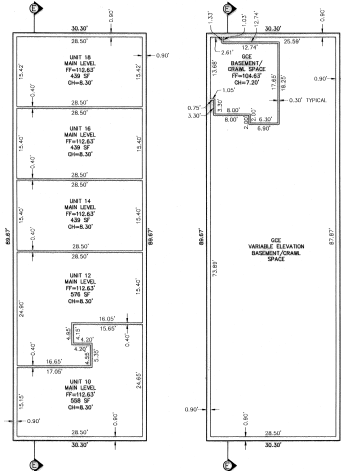
BUILDING 2601 SCALE: 1"=10'
